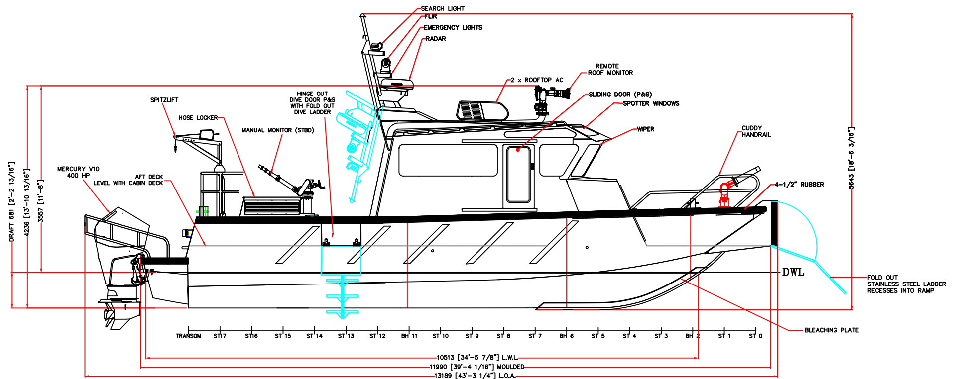
GENERAL ARRANGEMENT PROFILE VIEW
