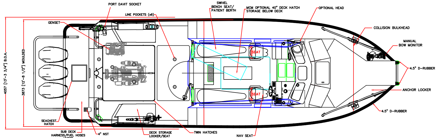
GENERAL ARRANGEMENT PLAN VIEW
